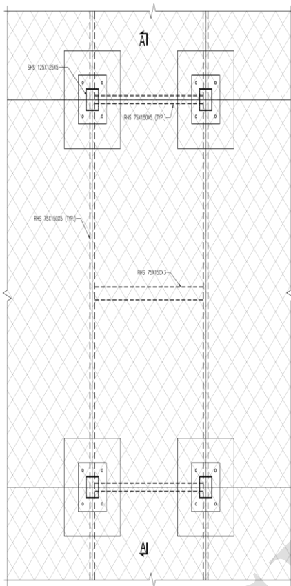
TYPICAL STRUCTURAL FRAMING PLAN TO SUPPORT SINGLE PANEL IN PORTRAIT ORIENTATION
