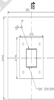
CONCRETE BLOCK DETAIL
